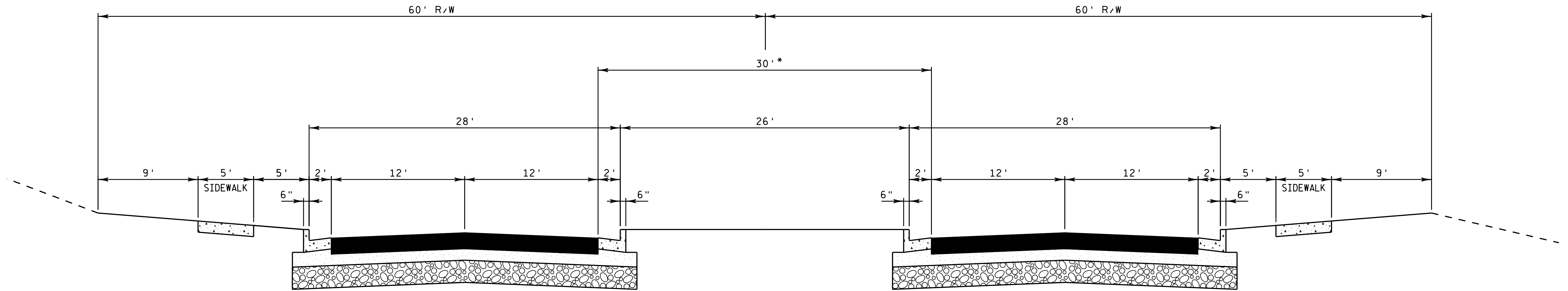
URBAN SECTION RAISED MEDIAN (DESIGN SPEED 40 MPH)
