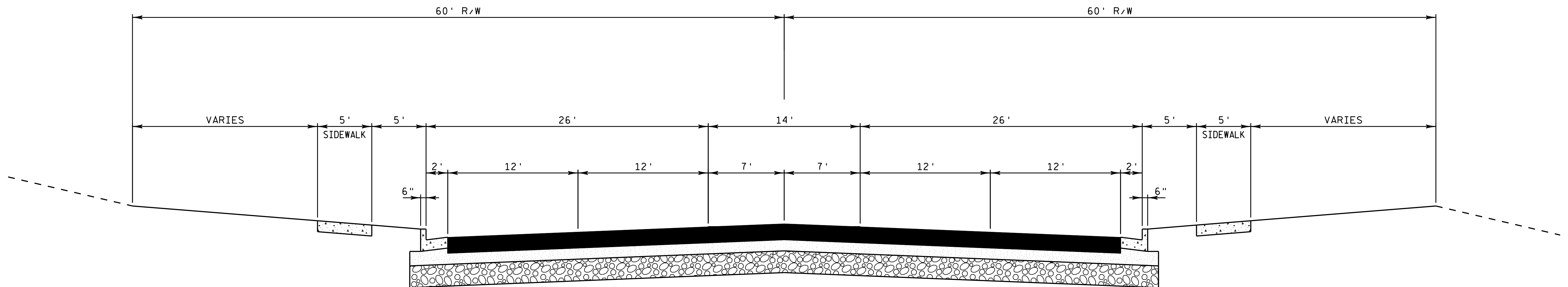
URBAN SECTION TWO-WAY LEFT TURN LANE (TWLTL) (DESIGN SPEED 40 MPH)
