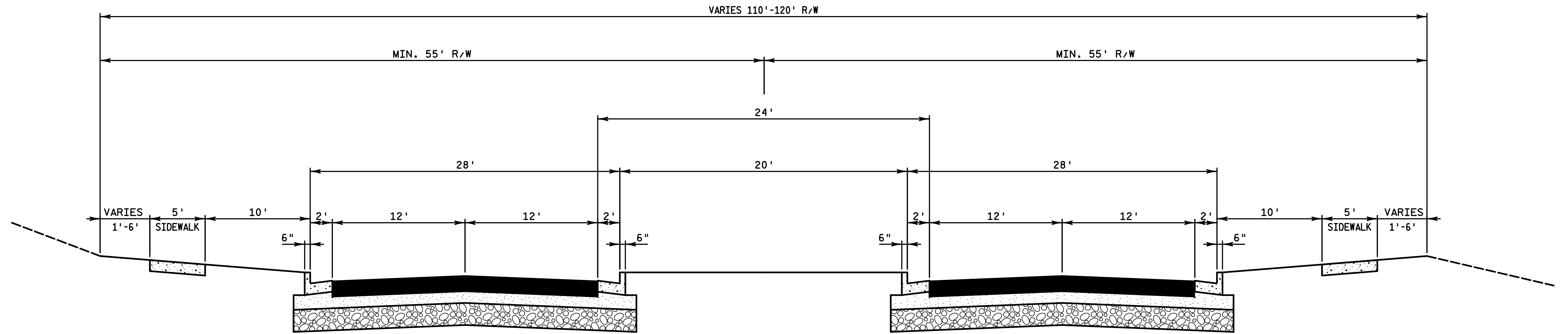
URBAN SECTION RAISED MEDIAN (DESIGN SPEED 40 MPH)
